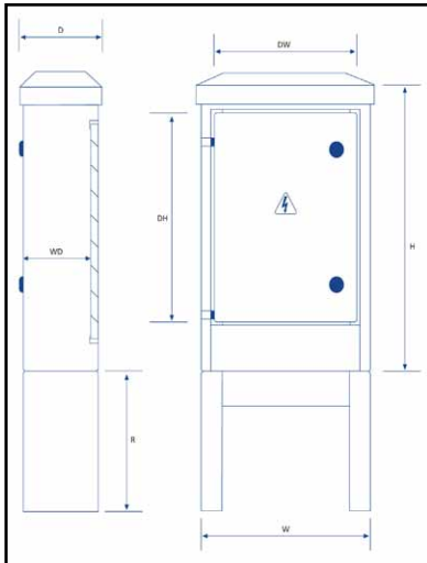
Dimensions (mm)
